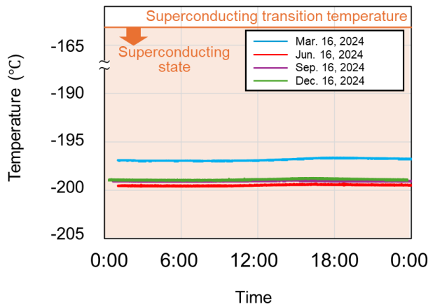
Fig. 2: Daily variation of cable temperature during superconducting feeding system operation
