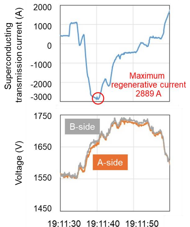
Fig.6: Examples of current and voltage during superconducting regenerative power supply
