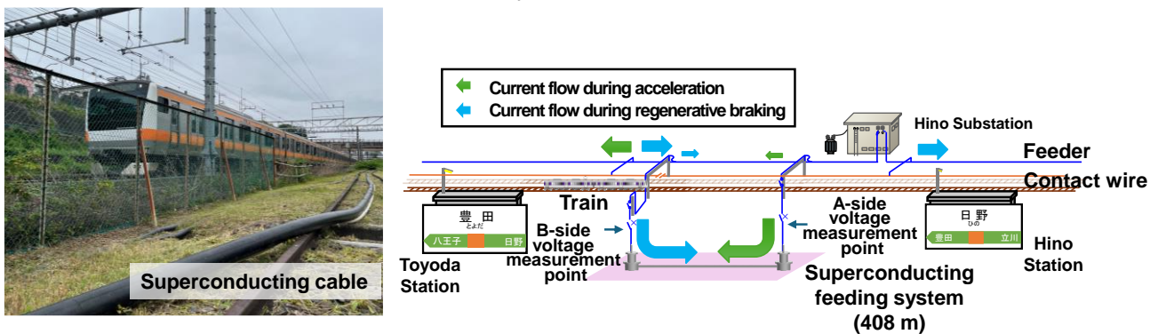
Fig. 4: Train running through power supply section using superconducting feeding system (high-current power supply on JR East Chuo Line)
