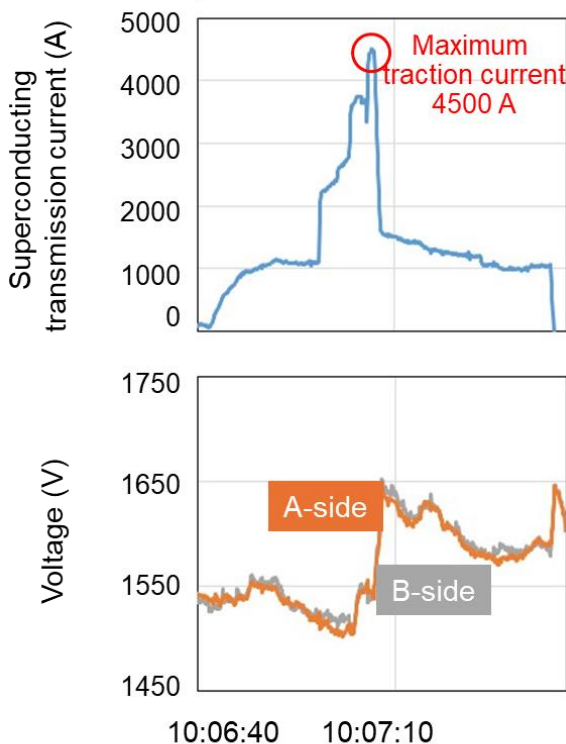
Fig.5: Examples of current and voltage during superconducting traction power supply
