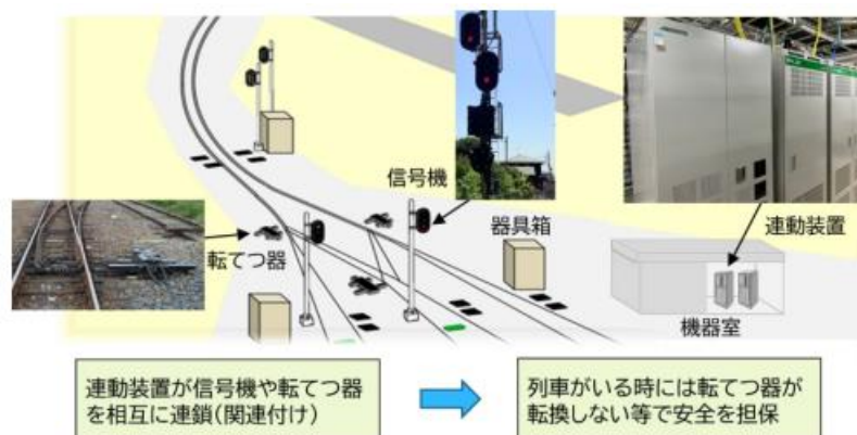
Figure-2 Interlocking equipment
